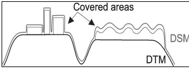
Figure 2. Difference between DTM (or DEM) and DSM
