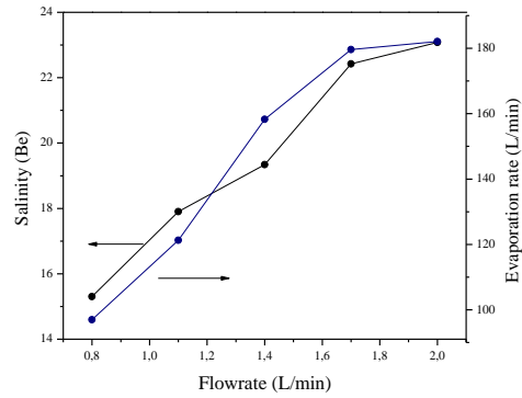
Fig. 2. Effect of flow rate to salinity and to evaporation rate at 90h evaporation time.
