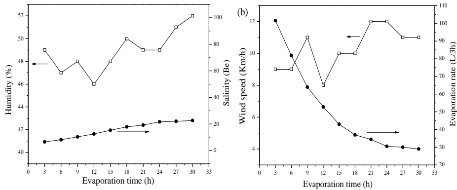
Fig. 1. Correlation of evaporation time to (a) humidity and salinity, and (b) wind speed and evaporation rate in the flow rate of 0.6 L/s.
