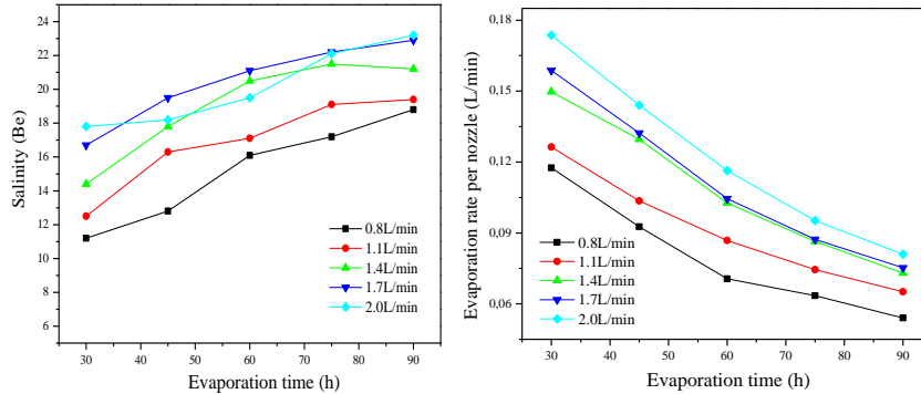
Fig. 4 Correlation of evaporation time to (a) salinity and (b) evaporation rate in the flow rate range of 0.8-2 L/min.
