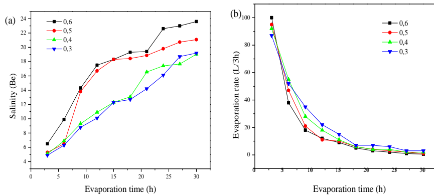
Fig. 3 Correlation of evaporation time to (a) salinity and (b) evaporation rate in the flow rate range of 0.3-0.6 L/s.
