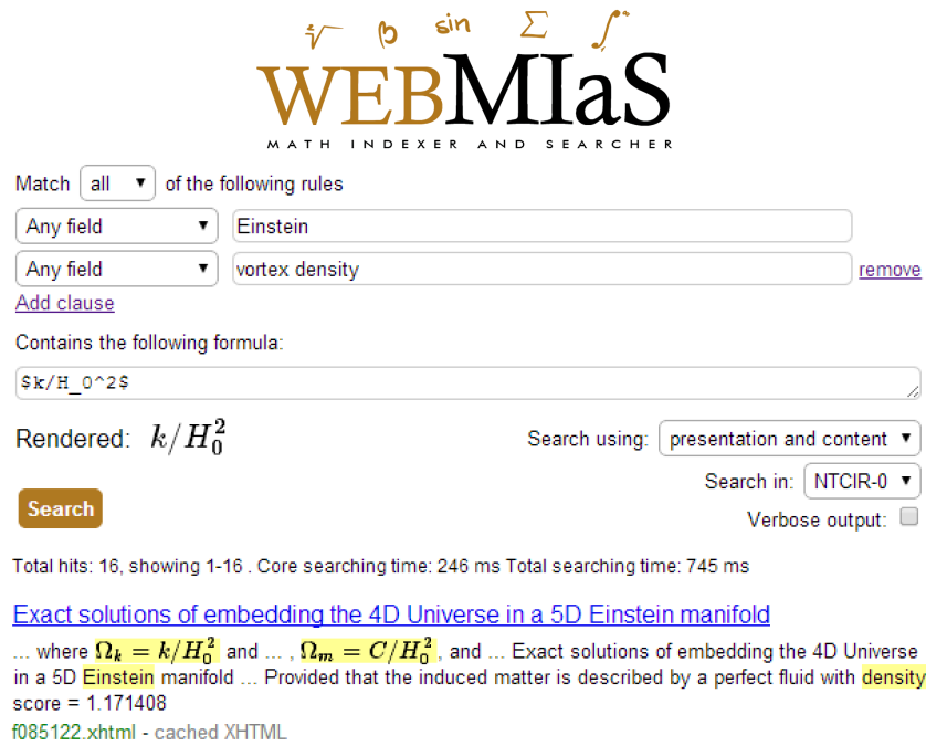
Fig. 2. Searching text and formulae with a single mixed query in WebMIaS.
