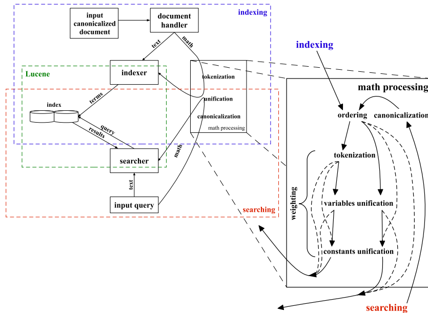
Fig. 1. The architecture of MIaS with indexing and searching phases overlapping over Lucene index. Besides standard text processing, the math input from indexing (a document) and searching (a query) stage is canonicalized, ordered, tokenized, and unified, afterward returned back to the indexer and searcher module, respectively.
