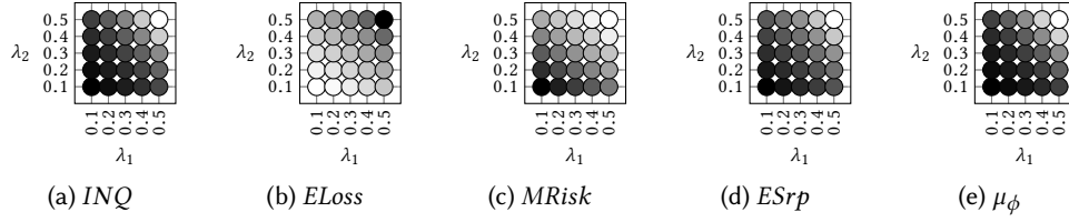
Fig. 3. We plot heatmaps of metrics for LP on GL-NYC with different combinations of hyperparameter settings ( \lambda_1, \lambda_2 ). Darker circles imply higher values of metrics at corresponding hyperparameter settings and lighter circles imply lower values. The darkest one represents the highest (out of all the trials with different settings) observed value of the corresponding metric and vice versa. Higher settings of \lambda_1, \lambda_2 can ensure better sustainability (fig-3a) but with slightly higher exposure loss for previously popular businesses (fig-3b), less risk for customers (fig-3c), and less amount of overexposure (fig-3d), but it costs loss in customer utility (fig-3e).
