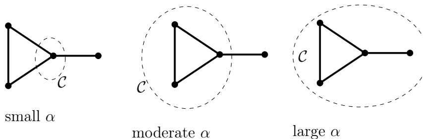
Fig. 6.3: The solutions of GTVMin (3.20) become increasingly clustered for increasing \alpha .
