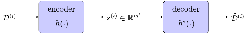
Fig. 7.2: An autoencoder consists of an encoder, mapping the input to a latent vector, and a decoder which tries to reconstruct the input as accurately as possible. The encoder and the decoder are trained jointly by minimizing some quantitative measure (a loss) of the reconstruction error (see [6, Ch. 9]). When using a local dataset as input, we can use the latent vector as its vector representation.
