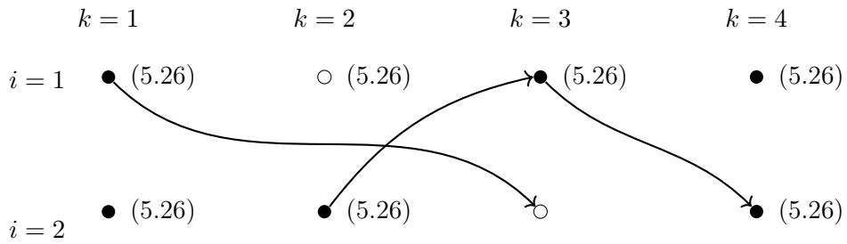
Fig. 5.4: Illustration of an asynchronous FL algorithm that results in a sequence of events, indexed by k = 1, 2, \dots . During event k , each active node i \in \mathcal{A}^{(k)} \subseteq \mathcal{V} of an FL network update their local model parameters \mathbf{w}^{(i)} by computing (5.26). We indicate the active nodes by filled circles.
