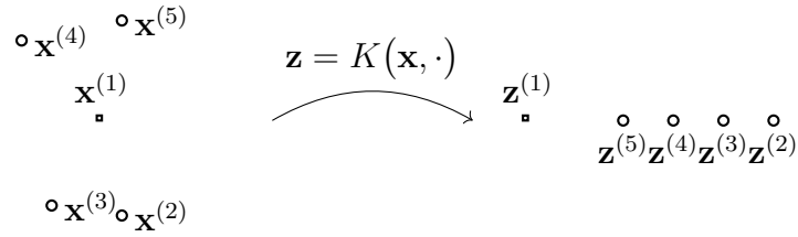
Fig. 10.6: Five data points characterized by feature vectors \mathbf{x}^{(r)} and labels y^{(r)} \in \{\circ, \square\} , for r = 1, \dots, 5 . With these feature vectors, there is no way to separate the two classes by a straight line (representing the decision boundary of a linear classifier). In contrast, the transformed feature vectors \mathbf{z}^{(r)} = K(\mathbf{x}^{(r)}, \cdot) allow to separate the data points using a linear classifier.
