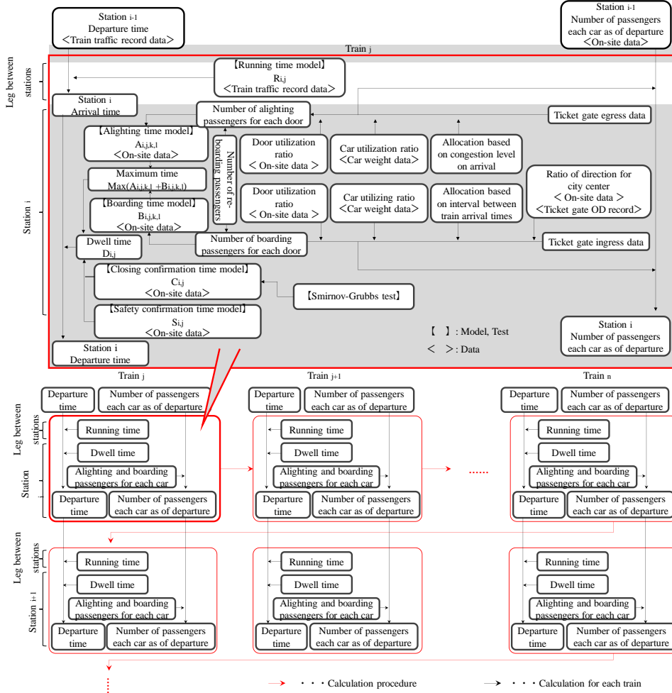
Figure 2: Simulation flow
