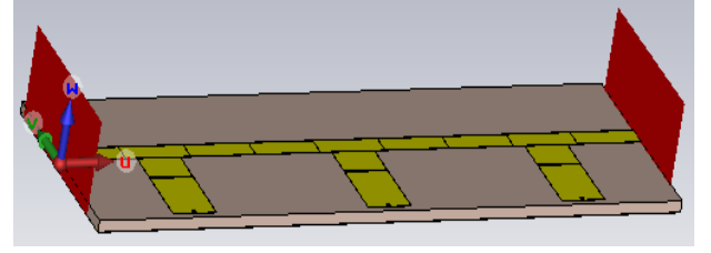
Fig. 1. Proposed microstrip low pass filter
