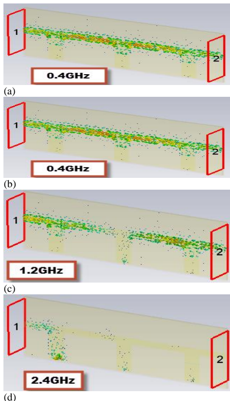
Fig. 7. Surface current at different field monitors
