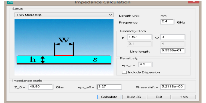
Fig. 5. CST Microwave studio impedance calculation
