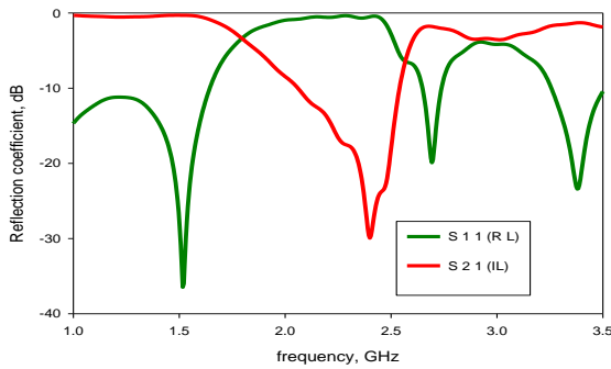
Fig. 6. Frequency response of the low-pass filter
