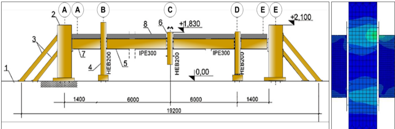
Figure 1 Frame specimen ,2 – stand resistance elements, 3- stand stabilizing elements, 4 –column, 5 –beam, 6 –middle column 7 – pin joint between frame side and column , 8 - reinforce concrete slab.
