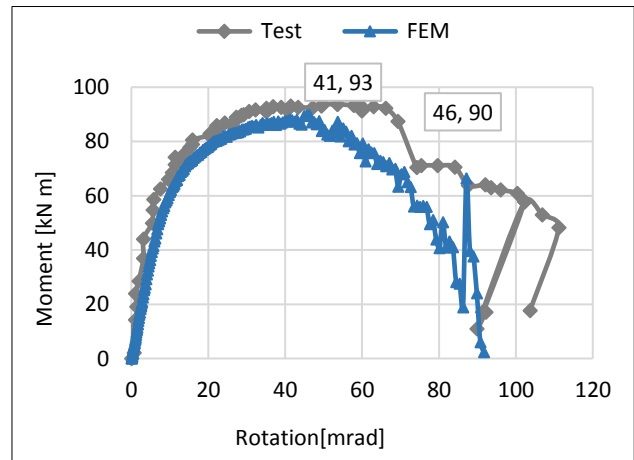
Figure 3 Moment-rotation curves form FE and Test for flush end-plate steel joints
