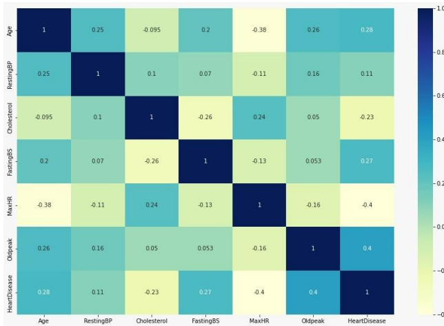
Fig 3. Correlation Matrix
