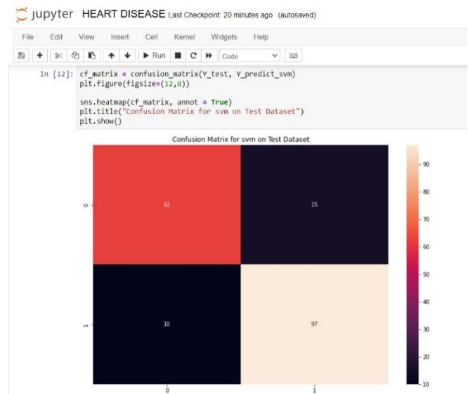
Fig 1. Confusion matrix
