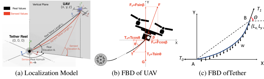
Fig. 5 Tether-based Localization [17]
