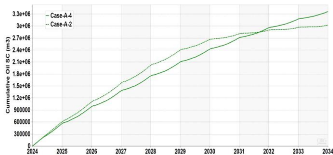
Figure 20: Cumulative oil production without AICV for the horizontal case (A-2) and the vertical case (A-4).
