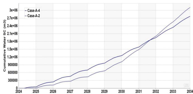
Figure 21: Cumulative water production without AICV for the horizontal case (A-2) and the vertical case (A-4).
