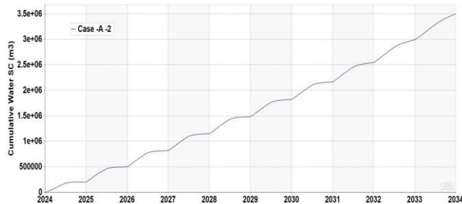
Figure 19: The field cumulative water volume for the modified case-A-2 with less well spacing distance.
