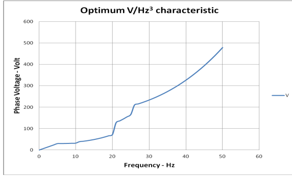
Fig. 4. Optimum V/Hz 3 Characteristic
