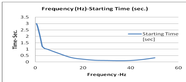
Fig. 13. Comparison Motor Starting Time Results
