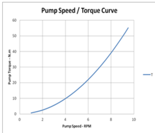
Fig. 2. Pump Speed/Torque
