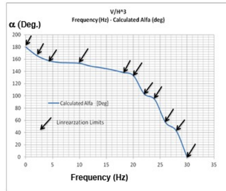
Fig. 6. Relations between firing angle “ \alpha ” and the “frequency based on V/Hz 3 Characteristic
