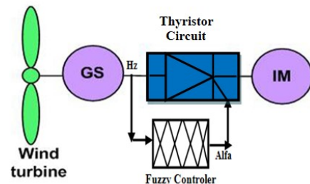
Fig. 1. System with voltage- frequency dependency fuzzy controller
