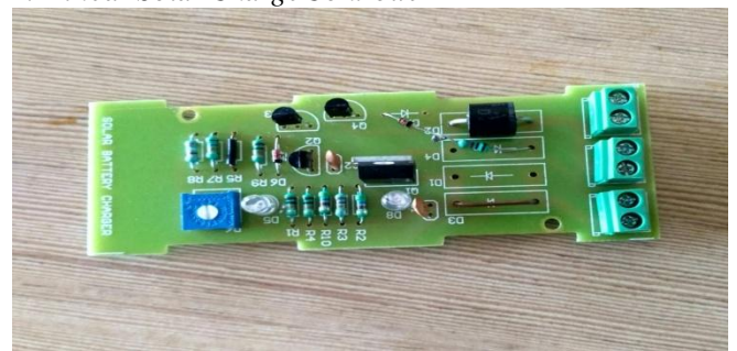
Fig.4 Linear Solar Charge Controller
