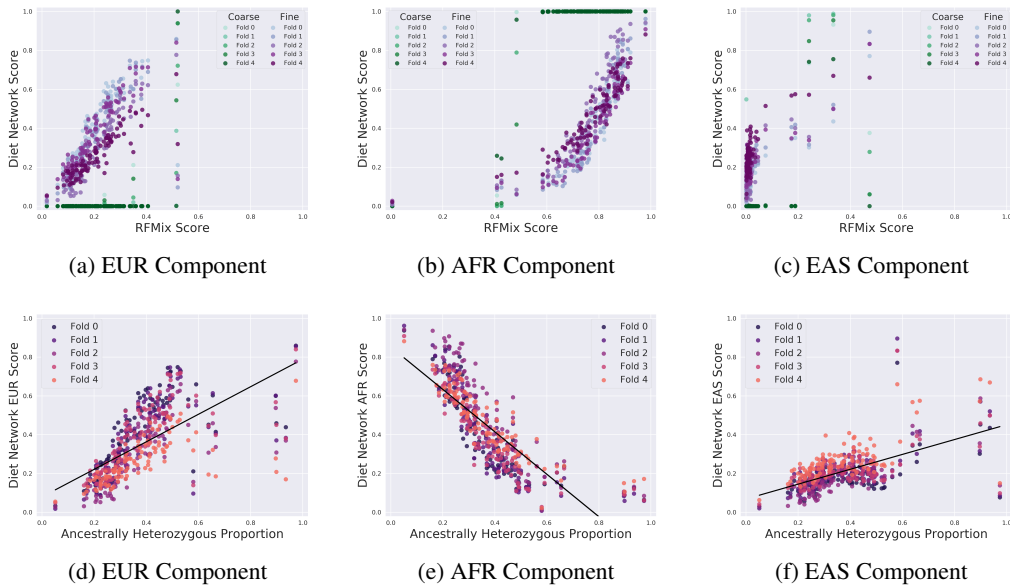
Figure 2: EUR(a), AFR(b) and EAS(c) scores for models trained on the 1000G dataset and tested on ASW compared to ancestry proportions inferred by RFMix. In purple are the scores returned by Model 2 ( fine ), in green by Model 3 ( coarse ). Correlation between fine model scores and RFMix proportions, from left to right, are r^2 = 0.63 , r^2 = 0.65 and r^2 = 0.61 . EUR(d), AFR(e) and EAS(f) scores returned by the fine model compared to the ancestrally heterozygous proportion (AHP) from RFMix. From left to right we have r^2 = 0.41 , r^2 = 0.66 and r^2 = 0.34 .
