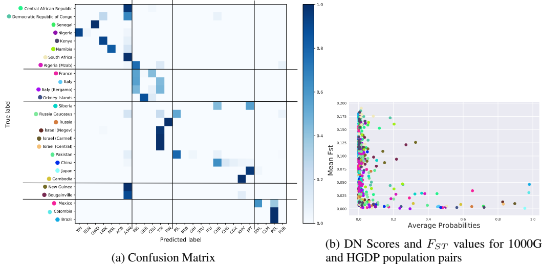
Figure 1: (a) Confusion matrix of classifications made by Model 1 tested on new individuals from the HGDP dataset. Since the DN model was trained using 5-fold cross validation, scores for HGDP individuals from all folds were averaged to get a single prediction by individual. True labels (y-axis) are not equivalent to the 1000G labels predicted by the network (x-axis). Black lines separate continental populations. (b) Relationship between DN scores and F_{ST} values for HGDP/1000G population pairs. DN scores were averaged on individuals from the same HGDP population. Each HGDP population is represented in the plot by 26 dots (see Fig. 1a for colors associated to HGDP populations). Each dot indicates the F_{ST} value between the given HGDP and a 1000G populations (y-axis) and the DN score for the 1000G population averaged on all individuals of the given HGDP population (x-axis).
