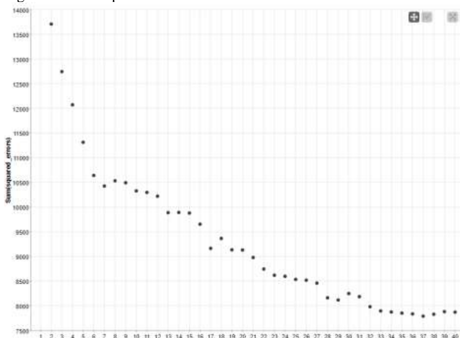
Figure 2. Scatter plot to determine the ideal number of clusters
