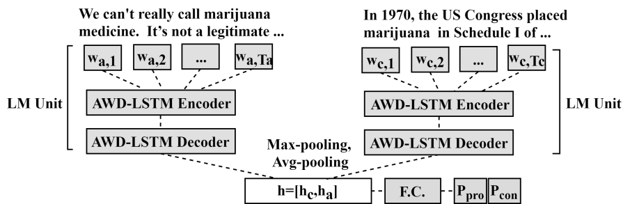
Fig. 1. The model; w_{a,i}, w_{c,i} i th word of argument and context sequence; F.C.: Fully Connected layer; p_{pro}, p_{con} : class probabilities; dark boxes use pretrained weights.
