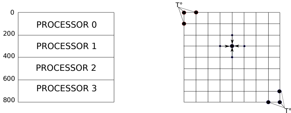
Figure 3: View of grid [800x800] partitioning according to the number of processors in this case 4 processors (left), example of the points involved when calculating heat at a point(right).
