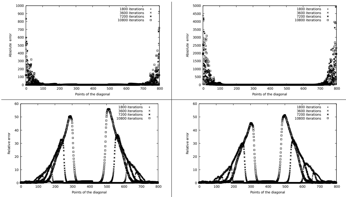
Figure 6: Absolute error and Relative error respectively between original program and optimized program, initial temperature: 1547.6^{\circ}\text{F} (top left, bottom left), for different iterations, initial temperature: 10106.6^{\circ}\text{F} (top right, bottom right).
