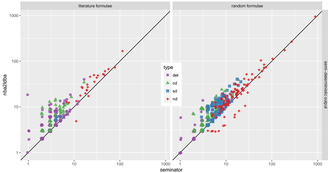
Figure 4: Comparison of the size of semi-deterministic automata produced by Seminador and nba2lba (both without reductions) on random formulae and on formulae from literature. Scatter plots are colored according to the output type of ltl2tgba -D . Scales are logarithmic.
